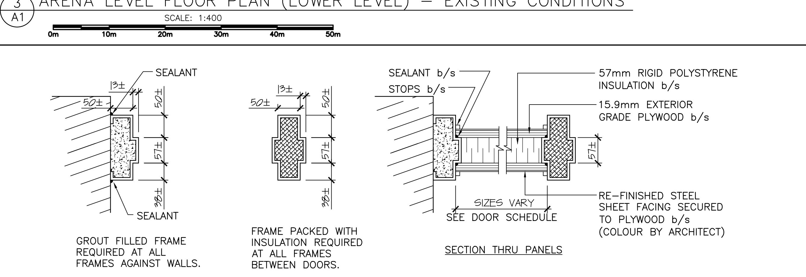
4 TYPICAL FRAME DETAILS SCALE: 1:5 0mm 100mm 200mm 300mm 400mm 500mm
